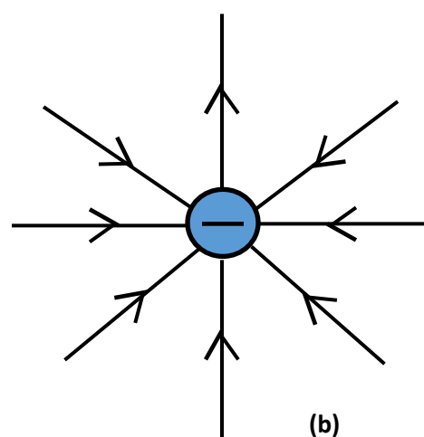
negative electric charge and field pointing radially inward
